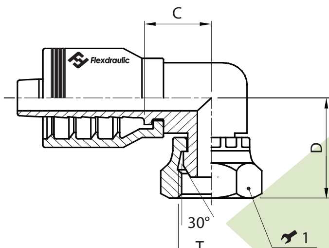
BSPP Female Swivel - 90° Compact Elbow (30° Cone Seat)
